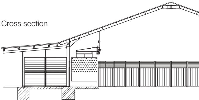
Triple combination: Round Stable with Gliding-Ring Horse Walker, paddock stalls and open interior at the Wiedmann Stud Farm
