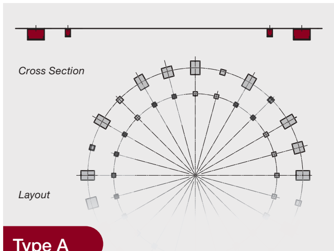
Independent footers
