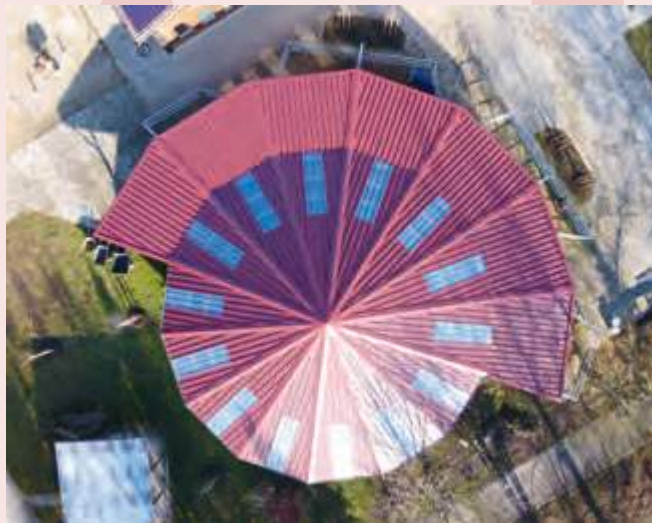
Ceiling-Mounted Horse Walker, Mendez, Mexico
