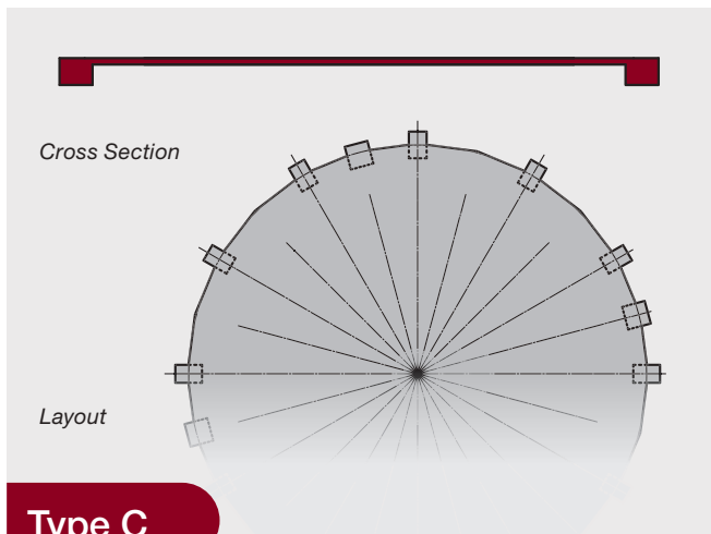
Individual foundations plus solid foundation
